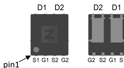
DFN5*6
